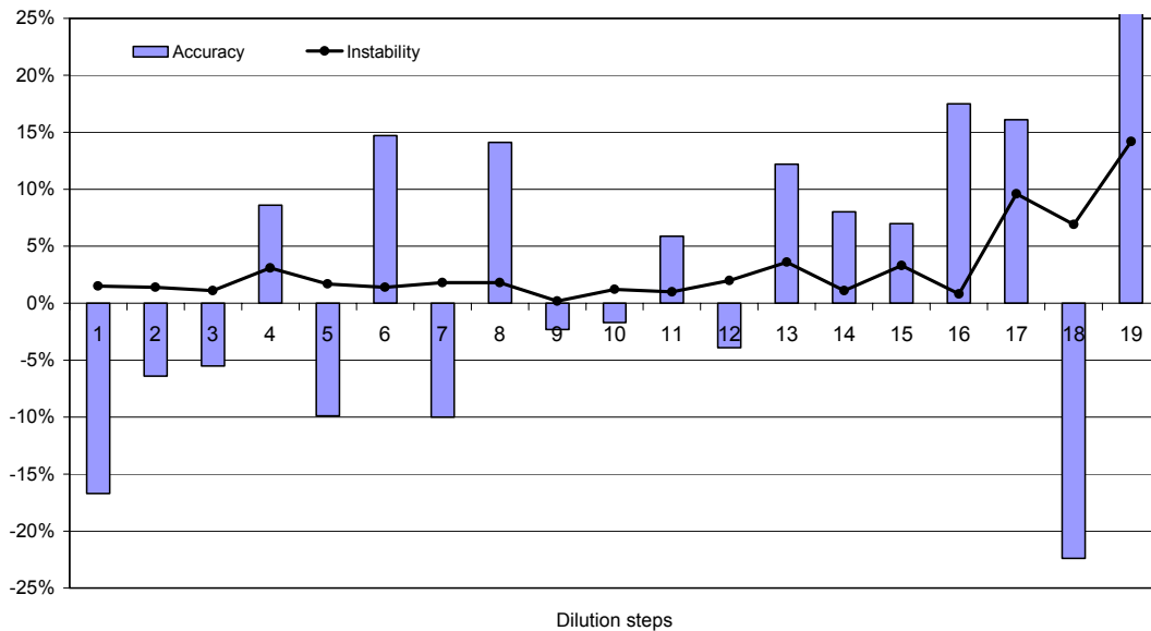
Figure 4 Accuracy and instability of the dynamic olfactometer
