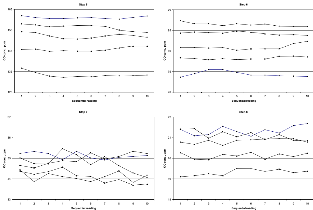
Figure 3 CO concentrations at dilution steps 5 – 8
